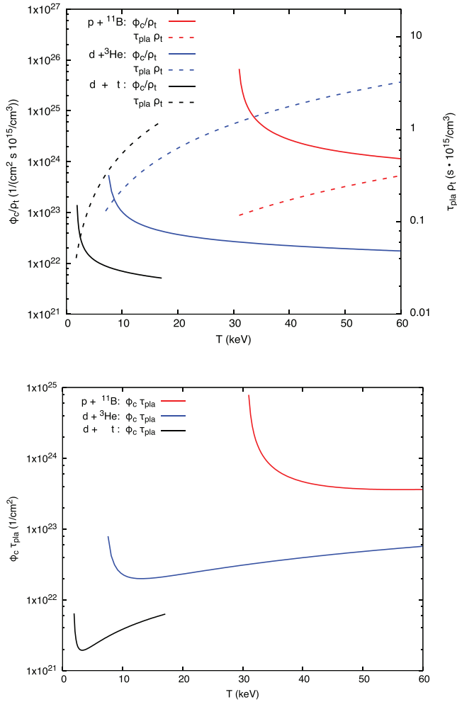
Figure 1. The critical flux divided by the plasma density \phi_c/\rho_t in units of 1/(\text{cm}^2 \text{ s } 10^{15} \text{ cm}^{-3}) and the associated plasma lifetime times its density \tau_{\text{pla}} \rho_t in units of \text{s} \cdot 10^{15} \text{ cm}^{-3} are plotted as a function of temperature for the three reactions in the upper panel. They terminate at T_{\text{max}} = 17.1 \text{ keV} for the d + t reaction. \phi_c \tau_{\text{phy}} is plotted as a function of T for the three reactions in the lower panel.
